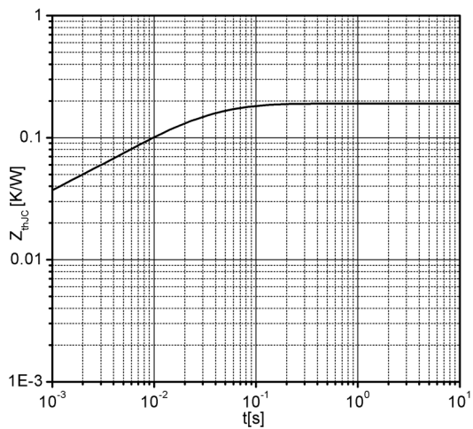
Fig 17. Typical Transient Thermal Impedance
